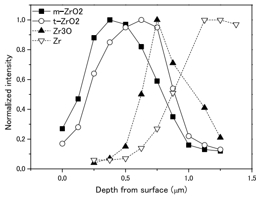
(a) FG-500°C-2h
