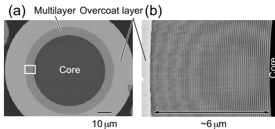
Fig. 2. Micrographs of the fabricated MZP obtained using a scanning electron microscope: (a) whole structure and (b) enlarged image of the multilayer region (region indicated by the white rectangle in (a)).
