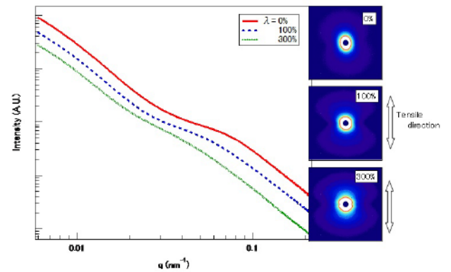
Fig. 2. SAXS profiles under tensile test.
