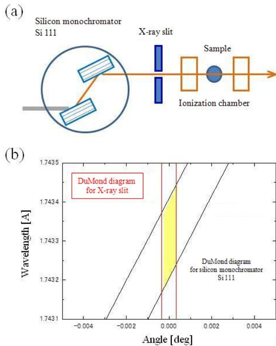
Fig. 12. (a) Schematic view of X-ray optics in a standard XAFS measurement case and (b) a DuMond diagram of the reflected X-rays.
