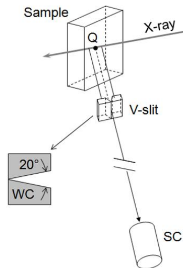
Fig. 1. Setup of microbeam X-ray diffraction for the 3D topography.
