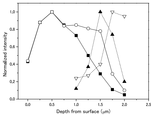
(e) FG-500°C-10h
