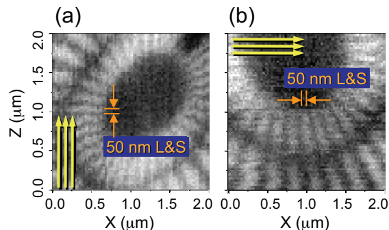
Fig. 6. Scanning transmission images of a Siemens star pattern. Yellow arrows indicate the scanning sequence.
