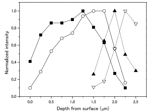
(f) AC-360°C-14days
