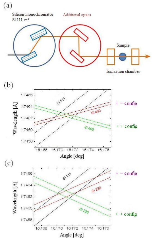
Fig. 13. (a) Schematic view of X-ray optics in a high-energy-resolution XAFS measurement case and DuMond diagrams of the reflected X-rays for (b) Si 111 + Si 400 reflections and (c) Si 111 + Si 220 reflections.
