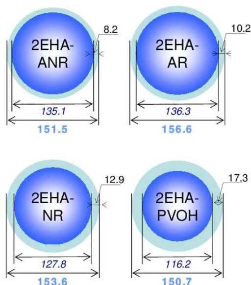
Fig. 1. Schematic models of the emulsion particles having the surfactants with various molecular length. Deep and light blue areas indicate the sizes of the core and the corona of the emulsion particles, respectively.
